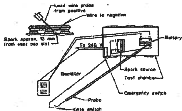
FIGURE P2 SCHEMATIC FOR TEST ON BATTERY
