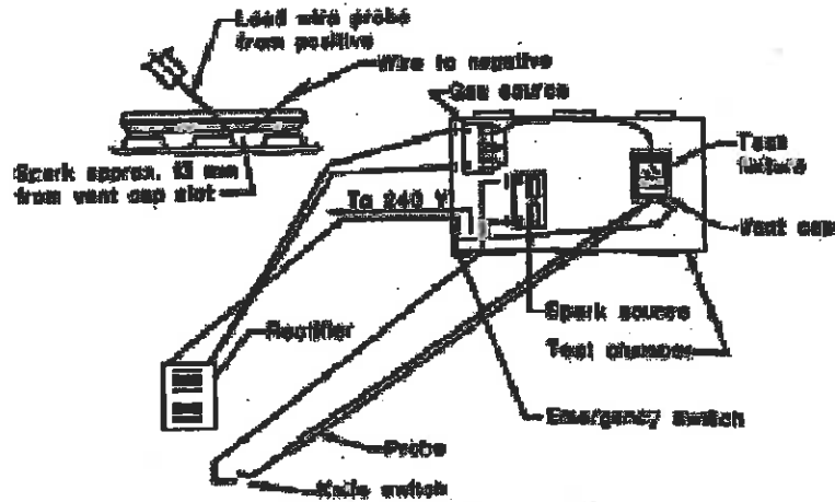
FIGURE P6 SCHEMATIC FOR TEST FIXTURE
